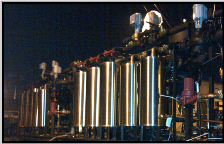
Triplex Skid Package: Heating-Hot Water-Pumping-Expansion-Air Separation
